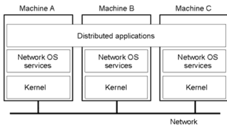
General structure of a network operating system.
